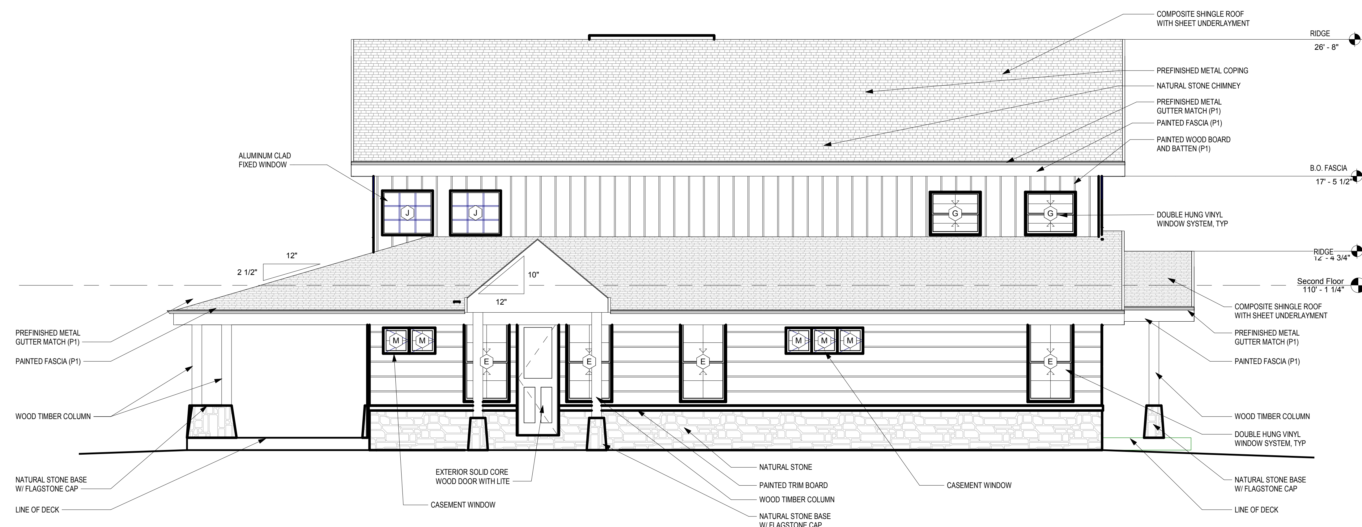
2 ENTRANCE ELEVATION 1/4" = 1'-0"
